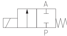
Anschlußplan / Connection diagram
